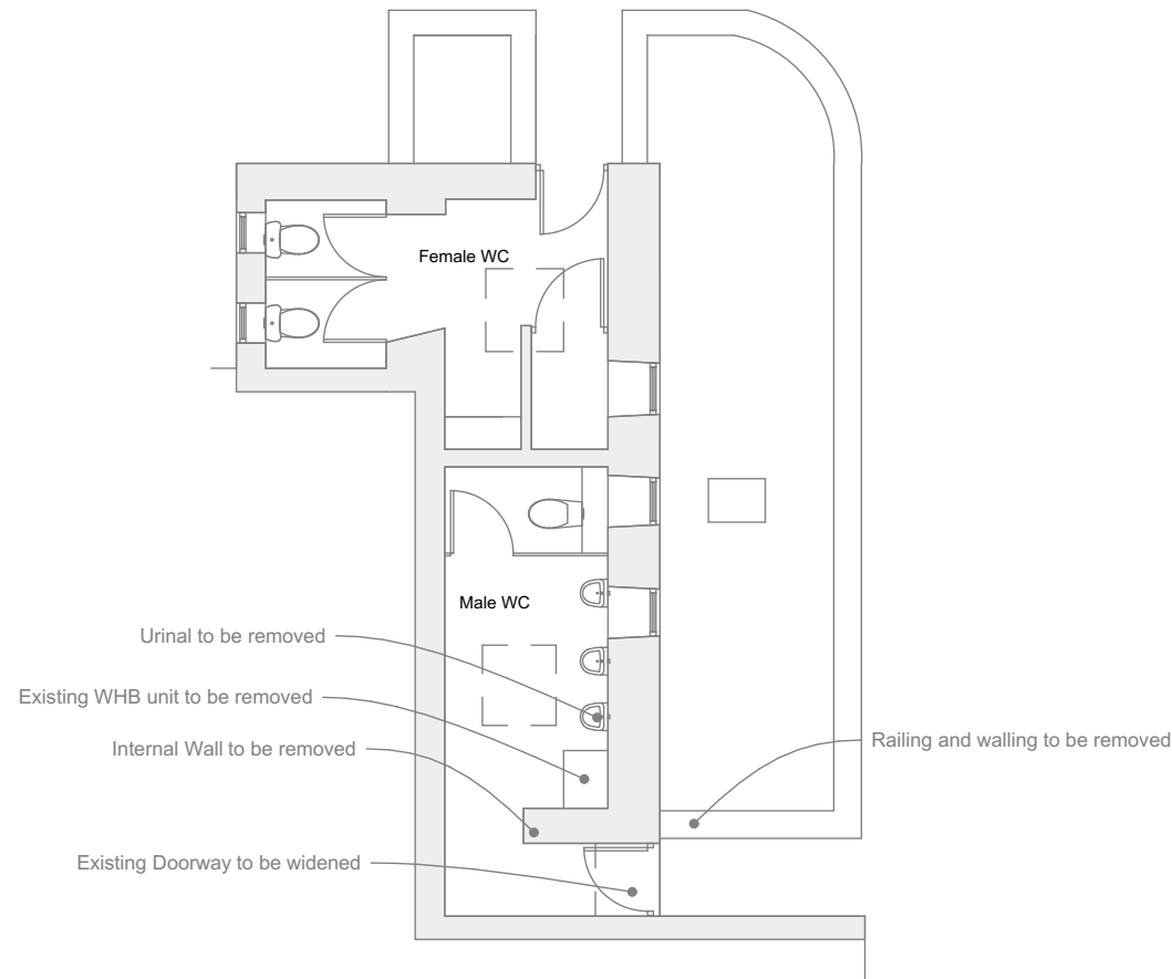
Floor Plan
