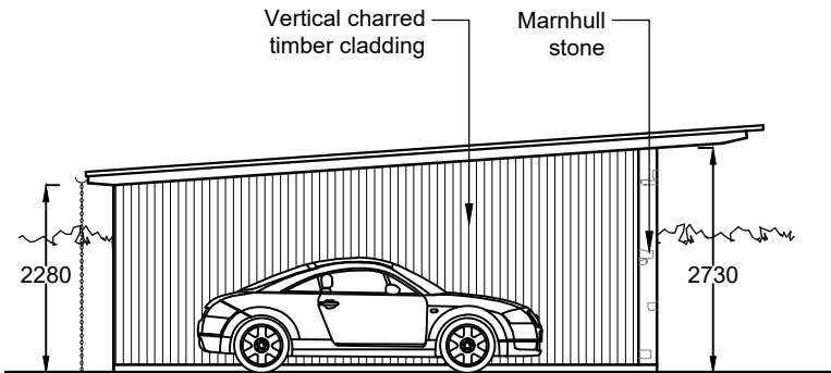
PROPOSED SECTION AA 1:100@A3
