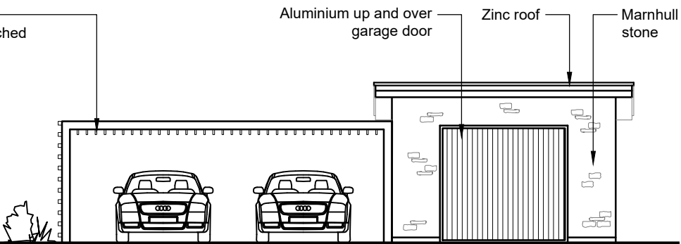
PROPOSED NORTH ELEVATION 1:100@A3
