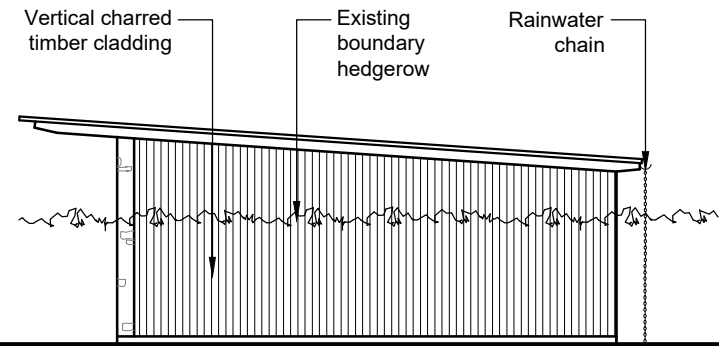
PROPOSED WEST ELEVATION 1:100@A3
