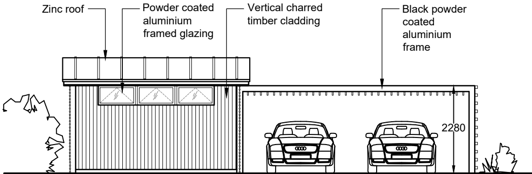
PROPOSED SOUTH ELEVATION 1:100@A3
