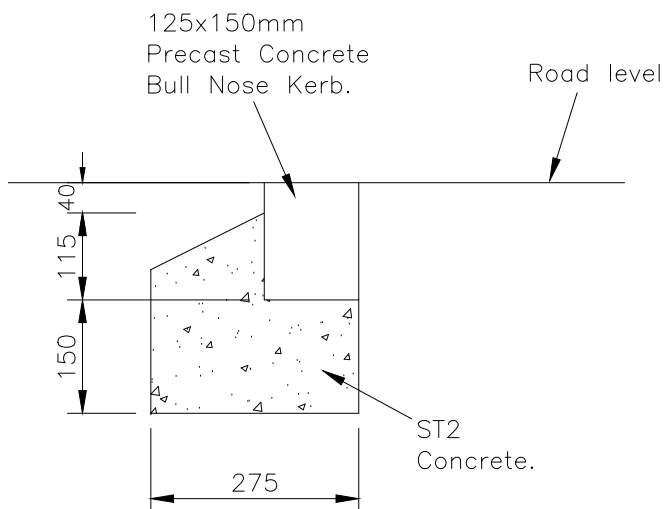
Kerb Detail
