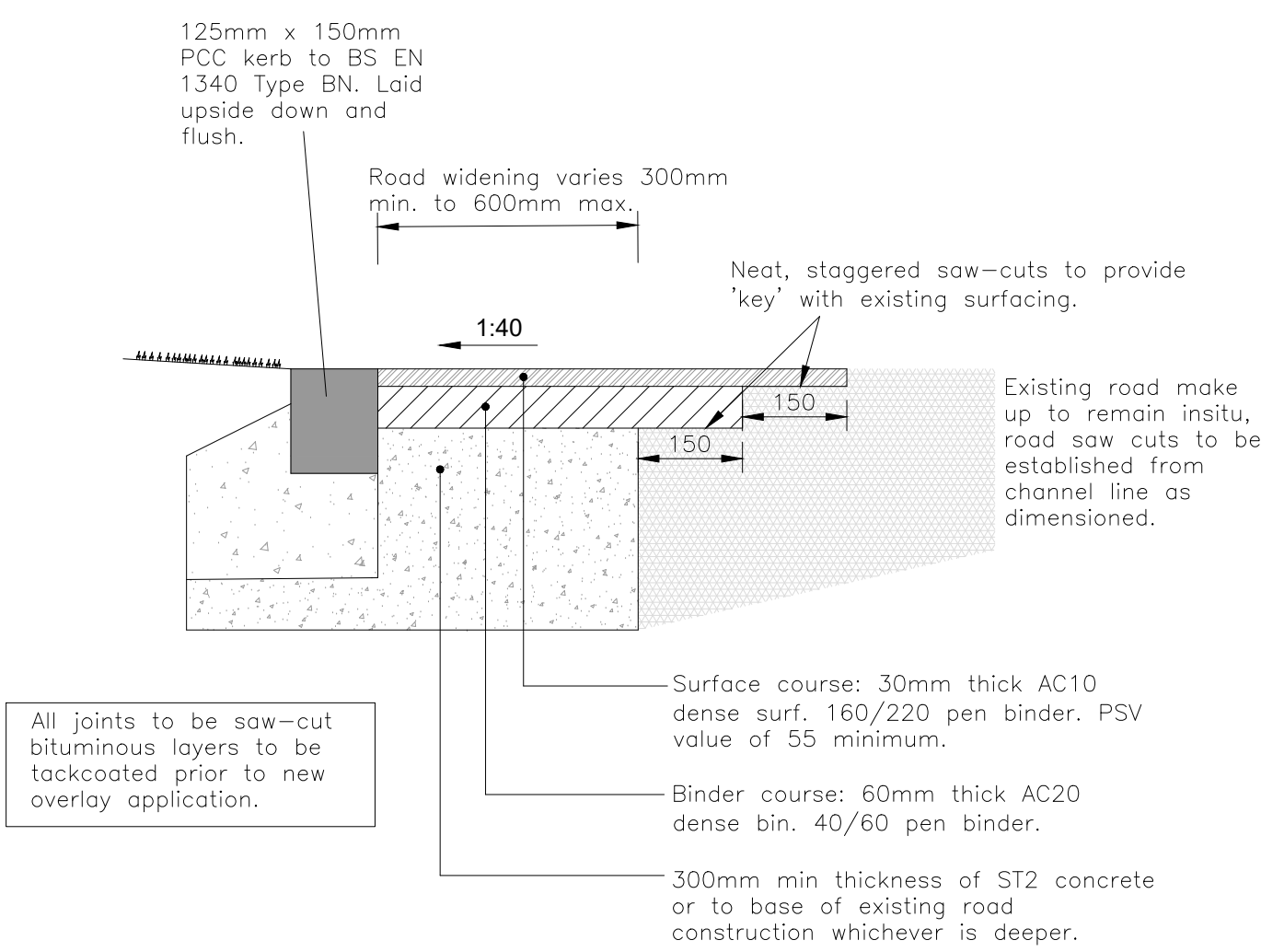
Narrow Carriageway Construction Applicable where widening of Existing Roads is <600mm wide. SCALE 1:10
