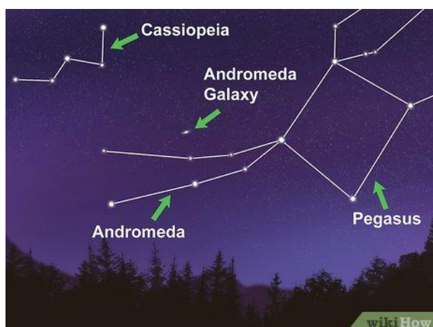
Pegasus and Andromeda
