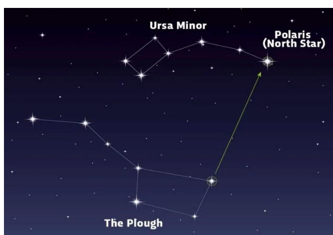
Finding Polaris and The Little Bear (Ursa Minor)
