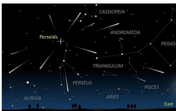
Perseids Radiant
