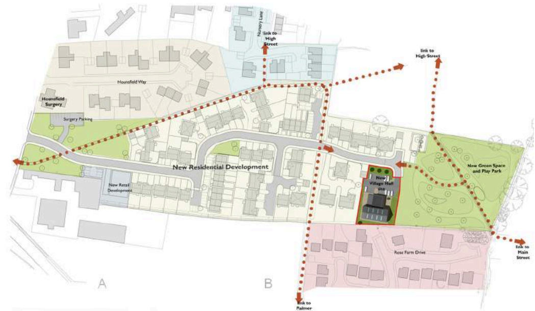
Location Plan
