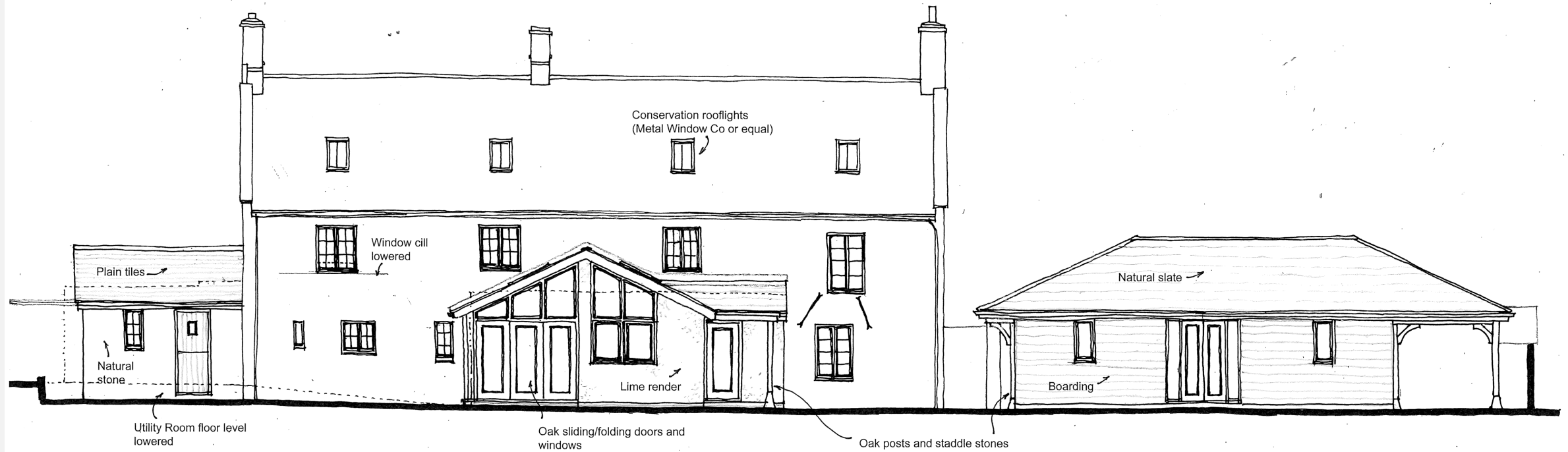
DRAFT REAR ELEVATION
